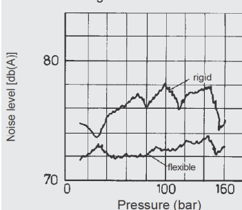
Noise level diagram
